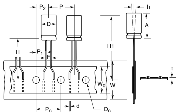
Fig. 2 - Straight Taping (5 \phi , 6.3 \phi , 8 \phi )
