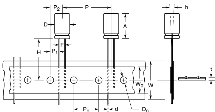
Fig. 4 - Straight Taping (16 \phi , 18 \phi )
