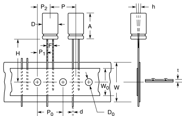
Fig. 3 - Straight Taping (Under 10 \phi , 12 \phi , 13 \phi )
